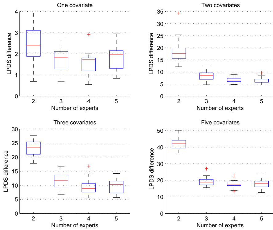
FIGURE 4. Simulated heteroscedastic data. Box plots of the difference in 5-fold cross-validated log predictive density score (LPDS) between the estimated SAGM(1) model and the SMR model as a function of the number of components in the SMR model. Each test sample contains 200 observations.
