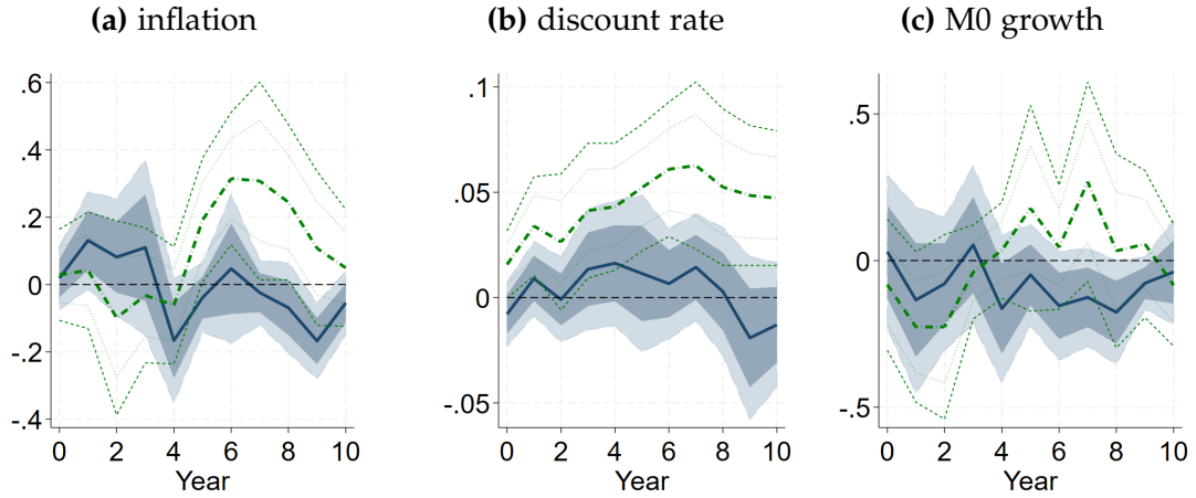
Figure 11: Impulse responses to terms of trade depreciation shock
