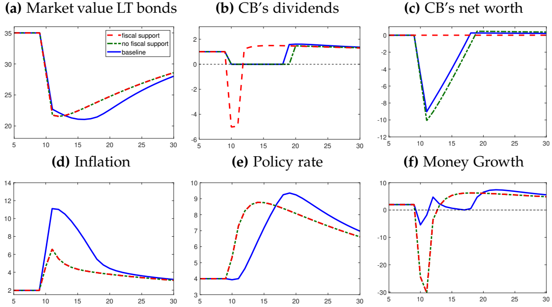
Figure 2: Impulse responses to a cost push shock
