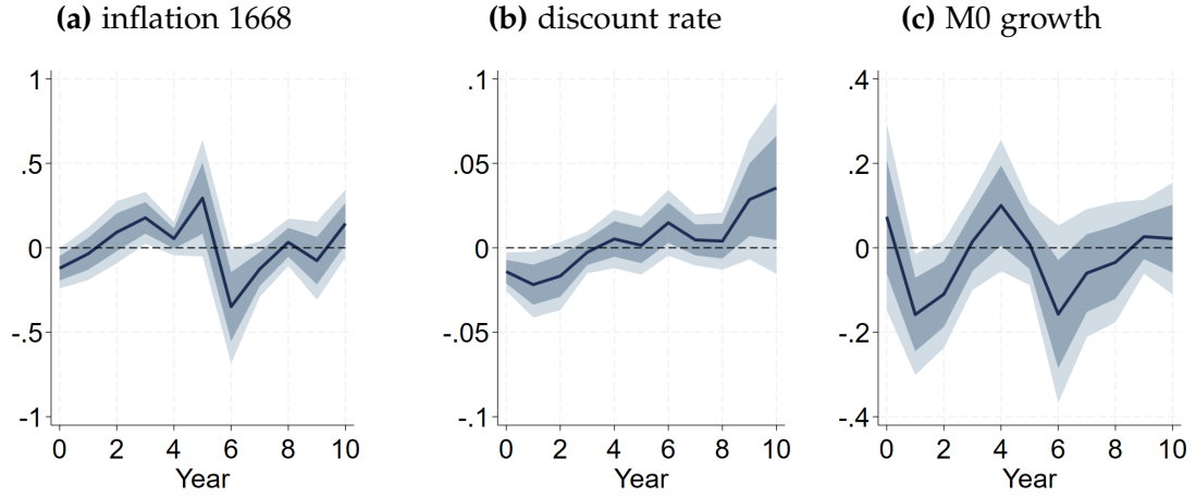
Figure B3: Inflation, discount rate and M0 growth response to quantitative profitability shocks, 1668-2023, all controls but primary deficit to debt
