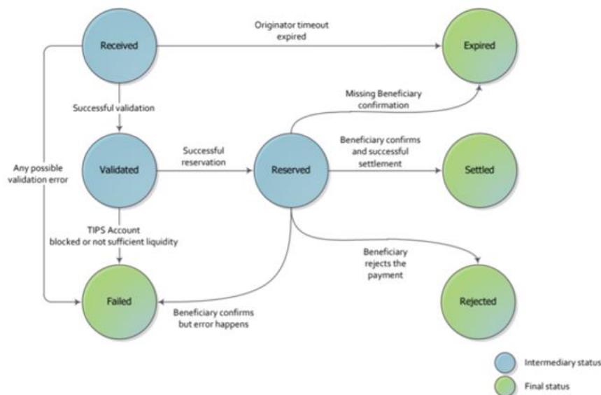
Illustration 38: Payment Transaction status transition diagram – Standard settlement model
