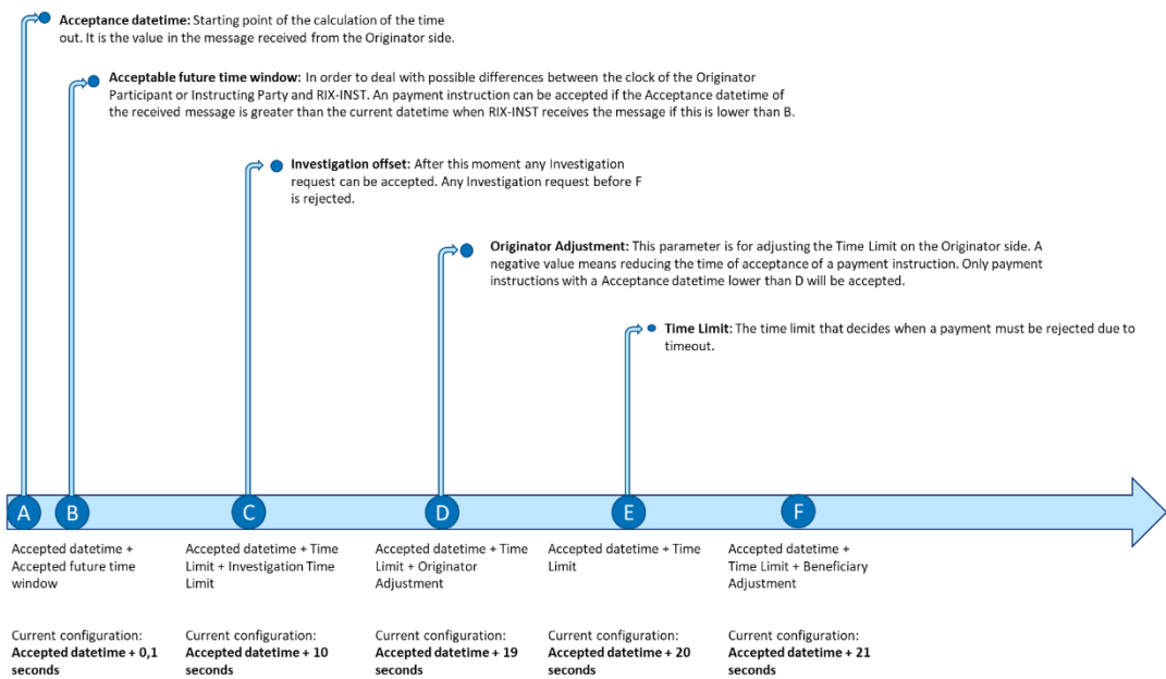
Illustration 17: Parameters for time limits
